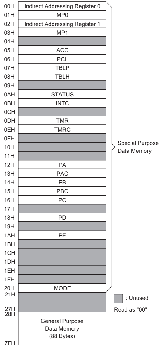
RAM Mapping
