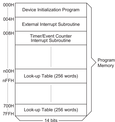
Program Memory for the HT48R52
