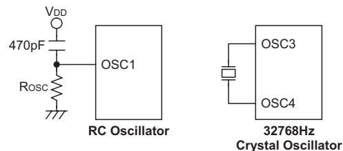
System Oscillator
