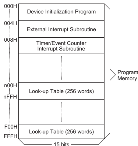
Program Memory for the HT48R53
