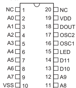
HT6012 -20 SOP-A
