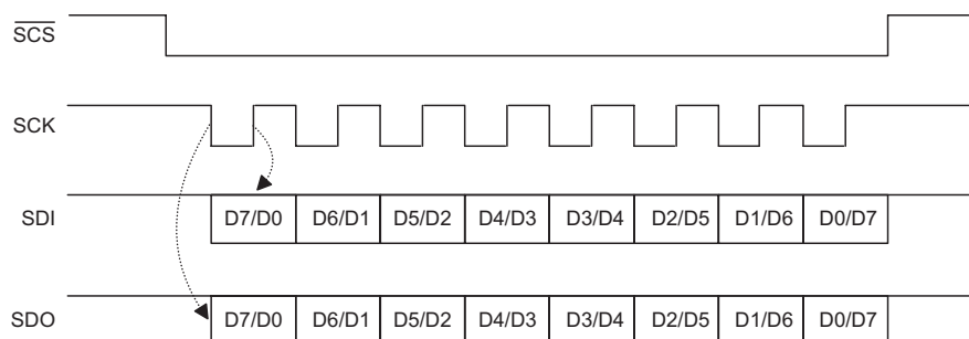
SPI Timing
