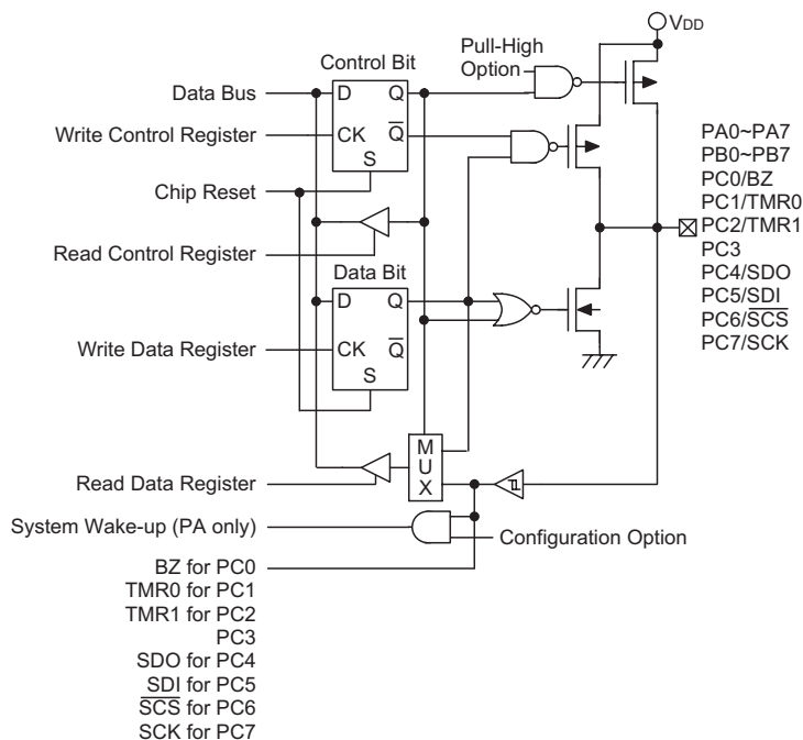
Input/Output Ports
