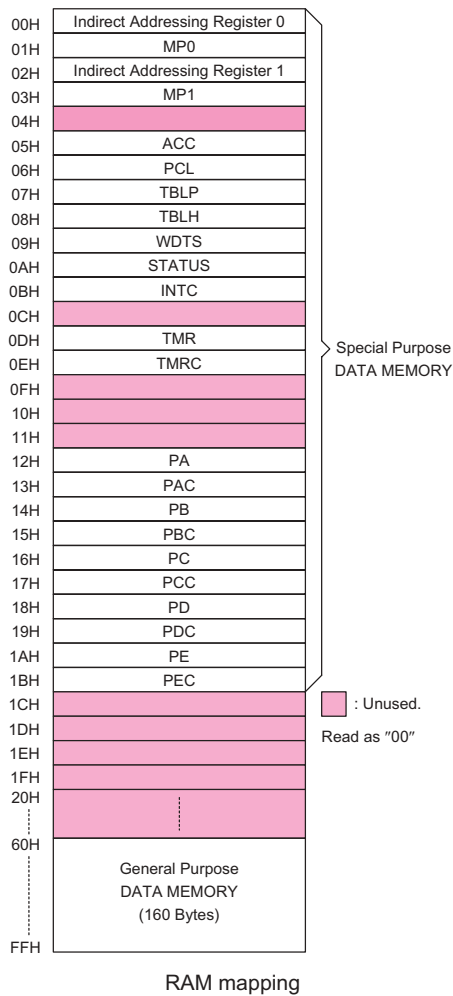
RAM mapping
