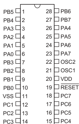
HT82K68A -28 SOP-A
