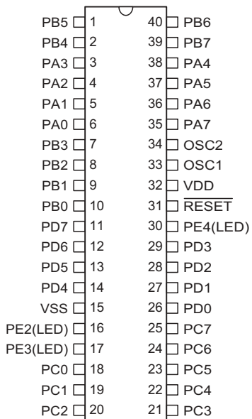
HT82K68A -40 DIP-A
