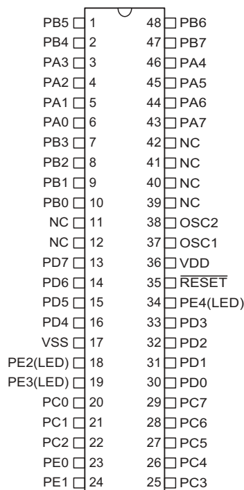
HT82K68A -48 SSOP-A
