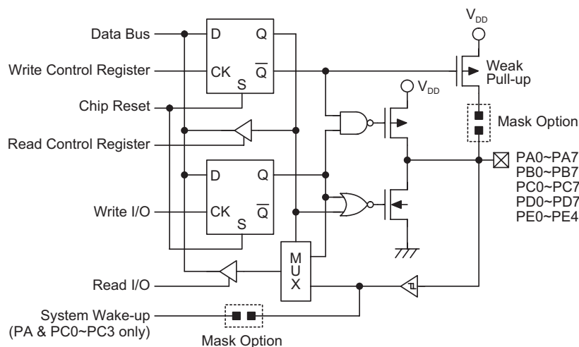
Input/Output Ports
