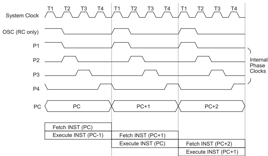
Execution Flow
