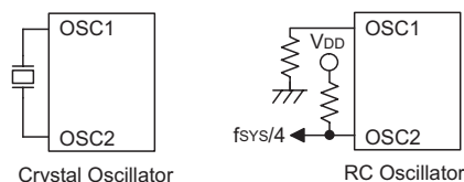
System Oscillator
