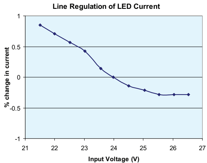
Fig. 2. Line Regulation of Output Current
