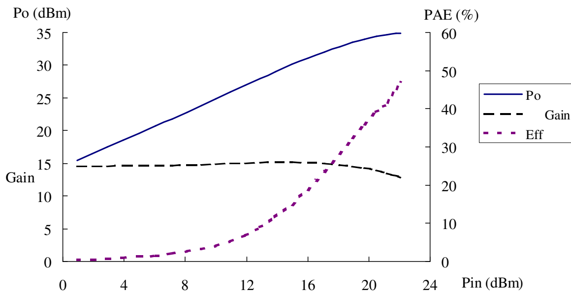
Output Power & Efficiency & Gain vs Input Power @ f=2.4\text{ GHz} , V_{ds}=10\text{V} , I_{ds} = 0.5 I_{dss}
