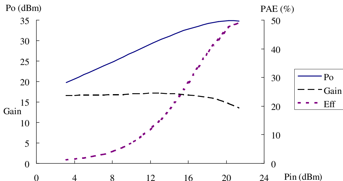
Output Power & Efficiency & Gain vs Input Power @ f=1.9\text{ GHz} , V_{ds}=10\text{V} , I_{ds} = 0.5 I_{dss}
