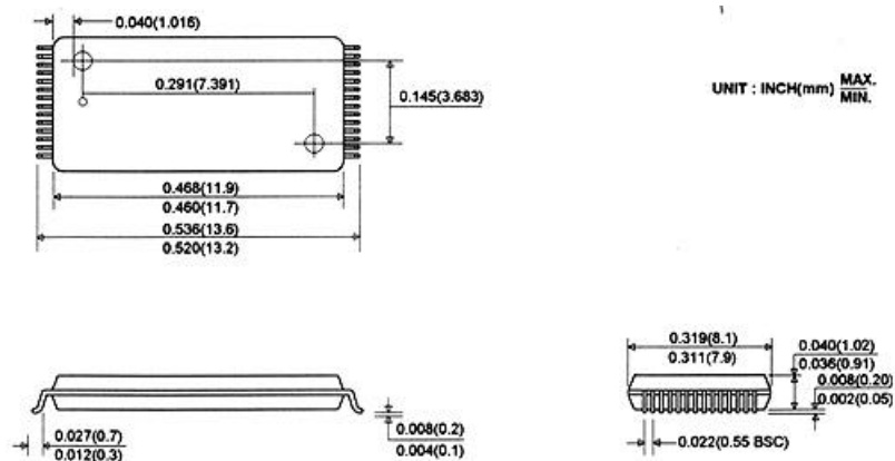
28pin 8X13.4mm Thin Small Outline Package SReversed(R1)
