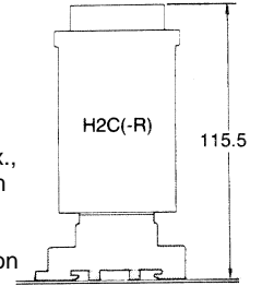
Mounting Height of Timer with Socket
