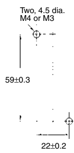
Mounting Holes
