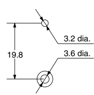
Mounting Holes (for Surface Mounting)
