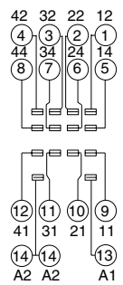
Terminal Arrangement
