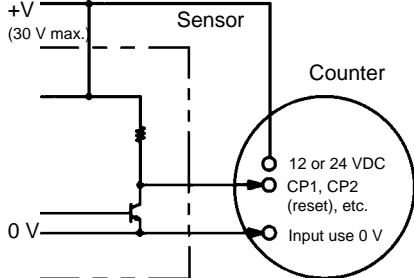
Solid-State Input (NPN output sensor powered by built-in DC power source)
