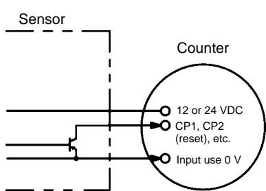
Solid-State Input (NPN transistor)
