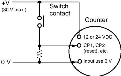
Contact Input
