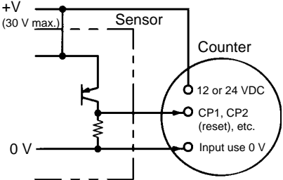
Solid-State Input (PNP transistor)
