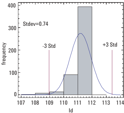
Figure 1. ID (mA) [7] Nominal = 111.2mA
