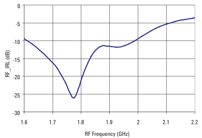
Figure 20. RF Return Loss vs. RF Frequency
