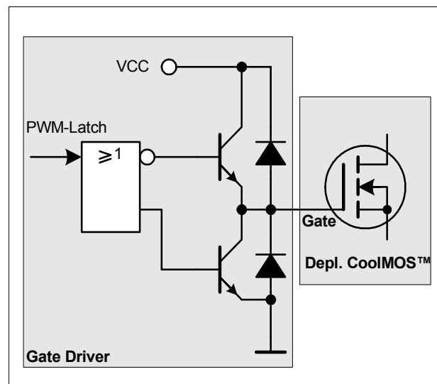
Figure 7 Gate Driver
