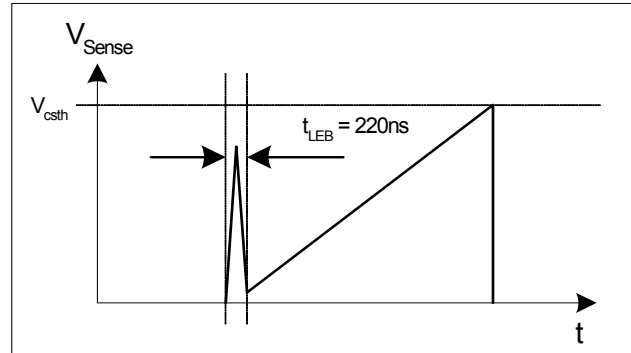
Figure 9 Leading Edge Blanking
