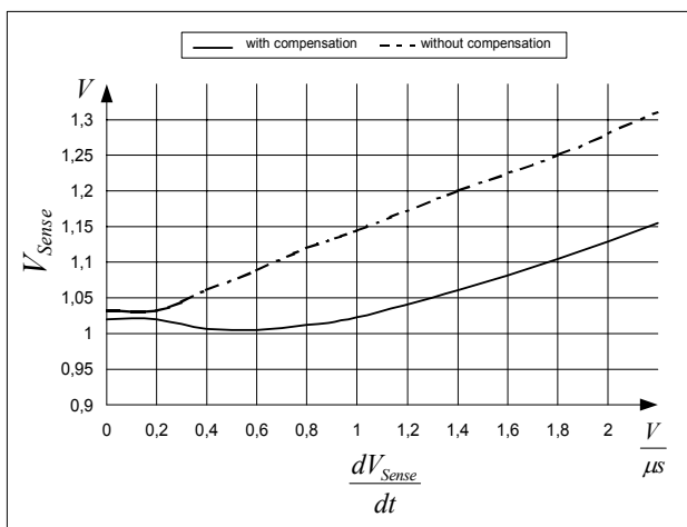
Figure 11 Overcurrent Shutdown
