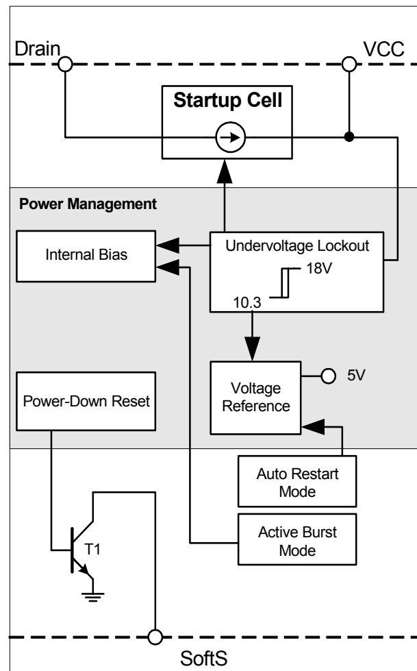
Figure 3 Power Management
