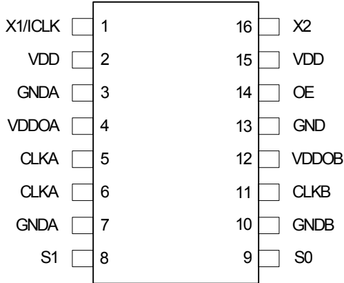
16-pin (173 mil) TSSOP
