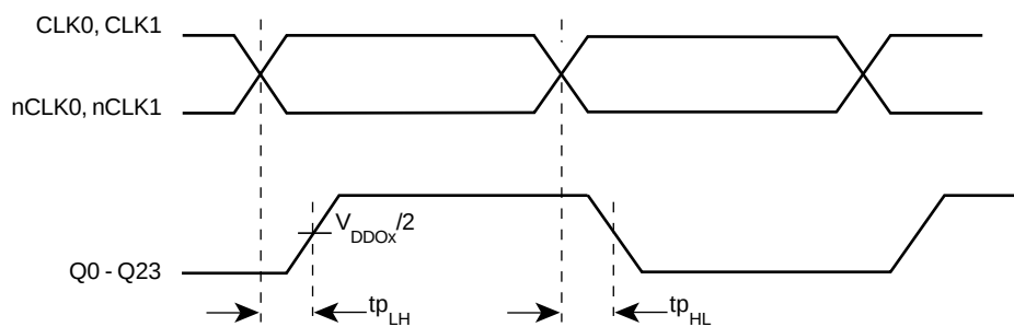
FIGURE 6 - PROPAGATION DELAY
