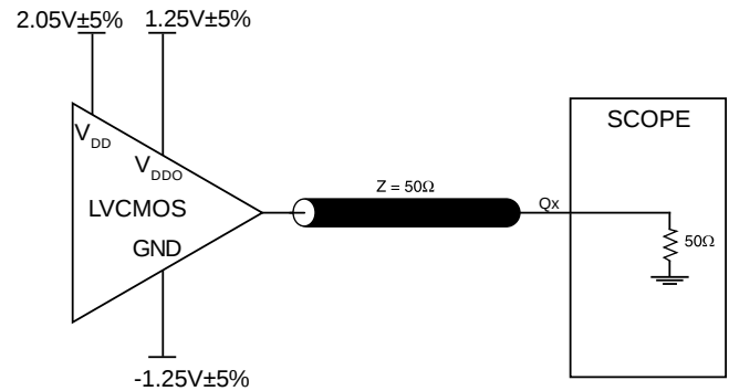
3.3V/2.5V OUTPUT LOAD AC TEST CIRCUIT
