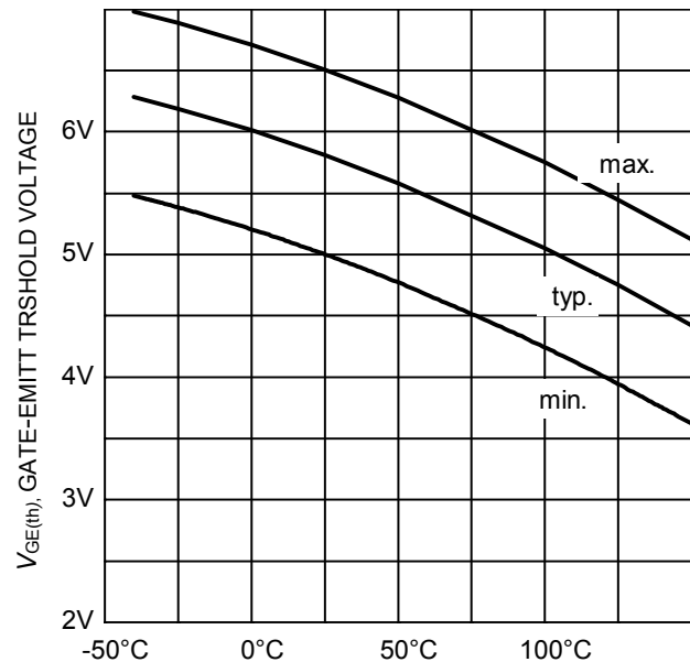
Figure 12. Gate-emitter threshold voltage as a function of junction temperature ( I_C = 0.7\text{mA} )
