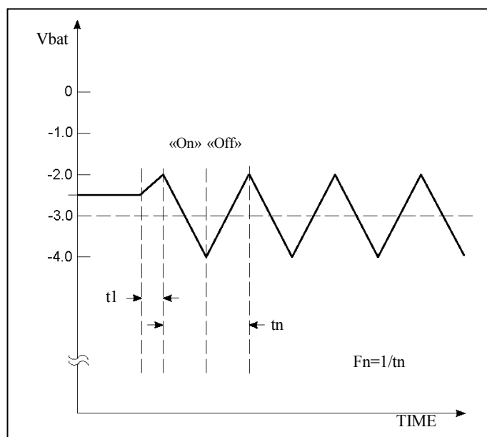
Figure 1 - Normal Operation Oscillator Timing Diagram
