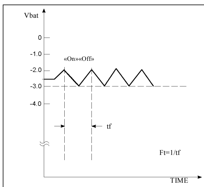
Figure 2 - One Defective Lamp Oscillator Timing Diagram
