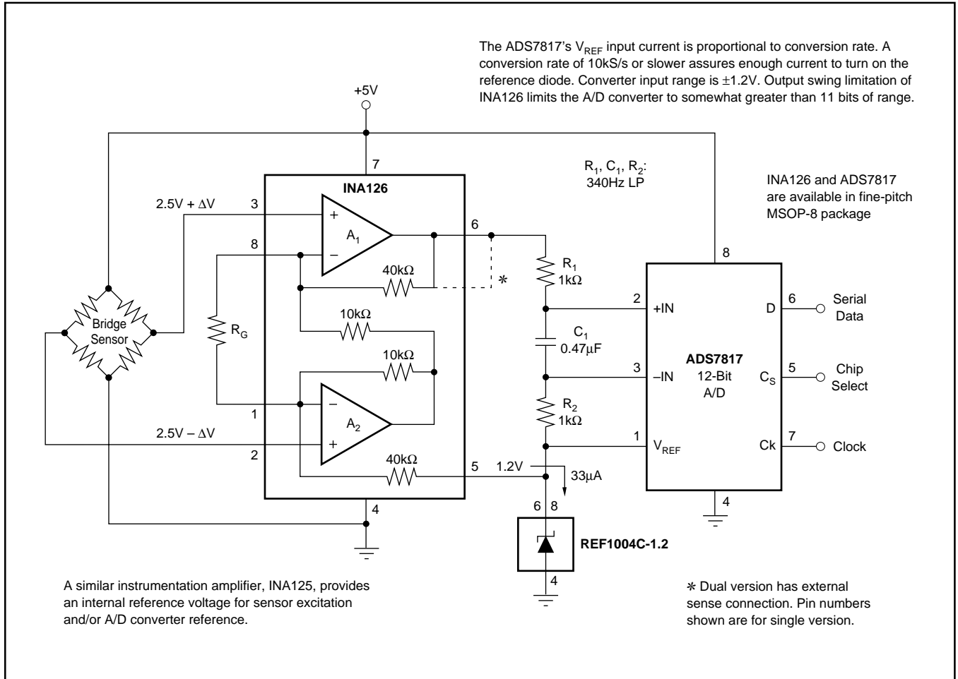
FIGURE 4. Bridge Signal Acquisition—Single 5V Supply.
