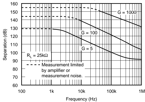
CHANNEL SEPARATION vs FREQUENCY, RTI (Dual Version)
