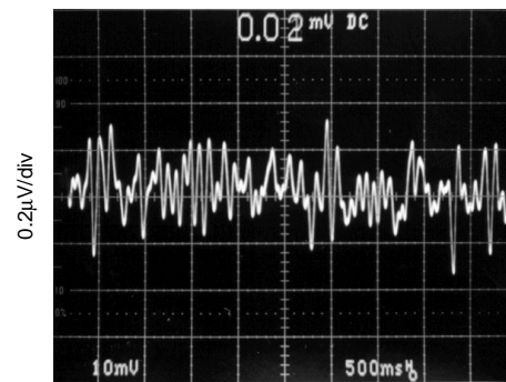
VOLTAGE NOISE, 0.1Hz to 10Hz
