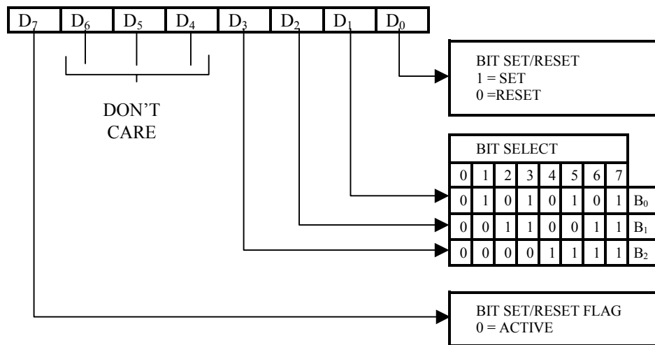
Figure 7. Bit Set/Reset Format
