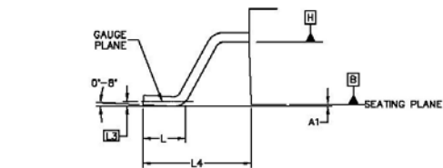
DETAIL "A" ROTATED 90° CW SCALE 8:1
