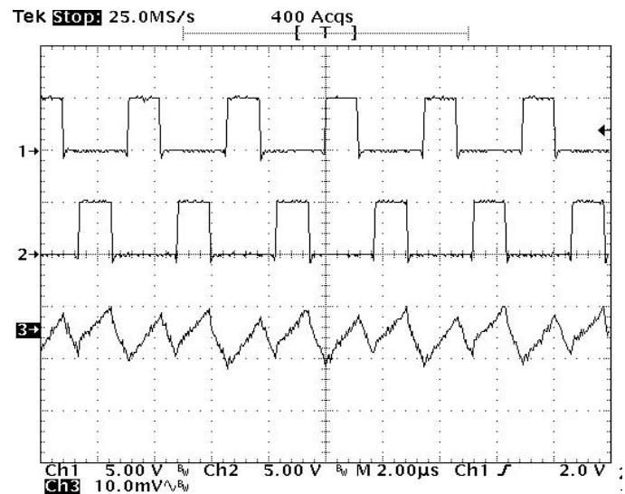
Fig. 28: iP1201PbF inductor current sharing
