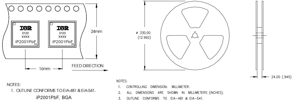
Fig.12: Tape & Reel Information
