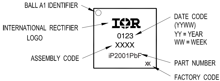
Fig.11: Part Marking
