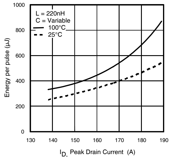
Fig 6. Typical E_{PII\_SF} vs. Drain Current
