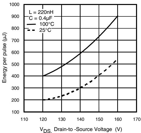
Fig 5. Typical E_{PII\_SF} vs. Drain-to-Source Voltage
