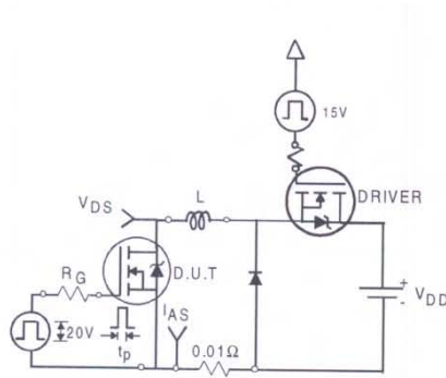
Fig 12a. Unclamped Inductive Test Circuit
