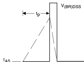
Fig 17b. Unclamped Inductive Waveforms
