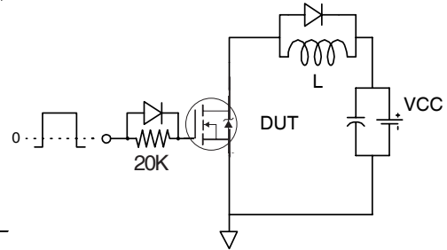
Fig 15. Gate Charge Test Circuit
