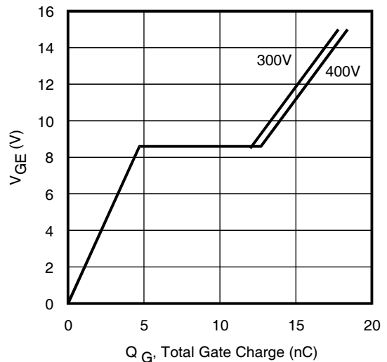
Fig. 24 - Typical V_{GE} vs. Q_G
