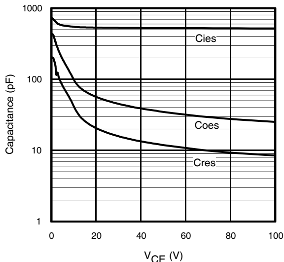
Fig. 23 - Typical Capacitance vs. V_{CE}
