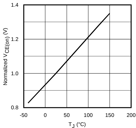
Fig. 18 - Normalized Typ. V_{CE(on)} vs. Junction Temperature
