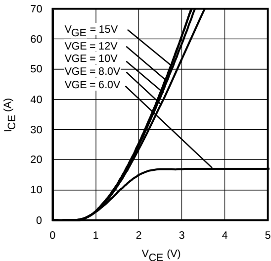
Fig. 5 - Typ. IGBT Output Characteristics
