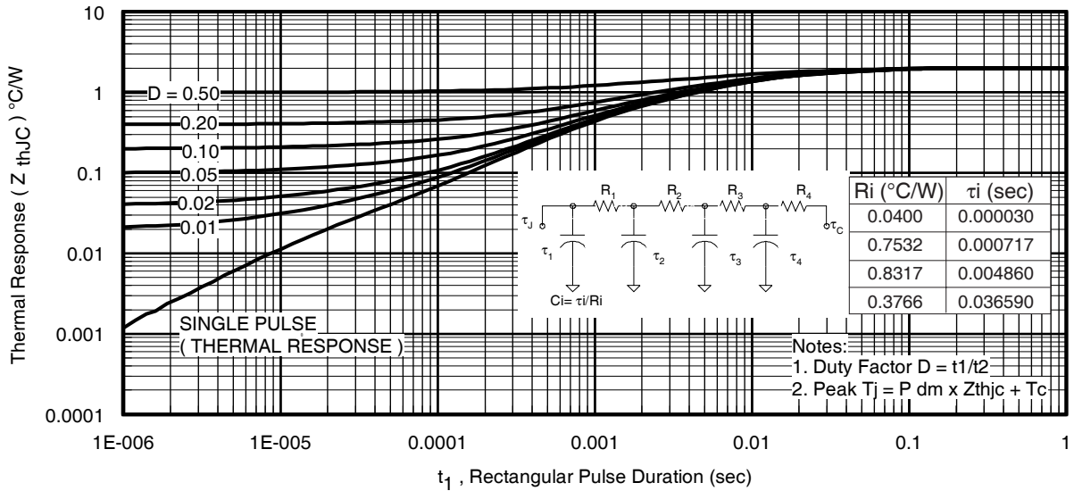
Fig. 20. Maximum Transient Thermal Impedance, Junction-to-Case (DIODE)
