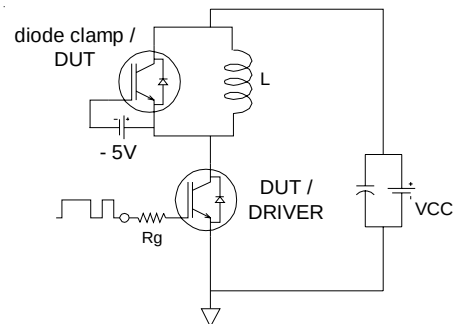
Fig.C.T.4 - RBSOA Circuit
