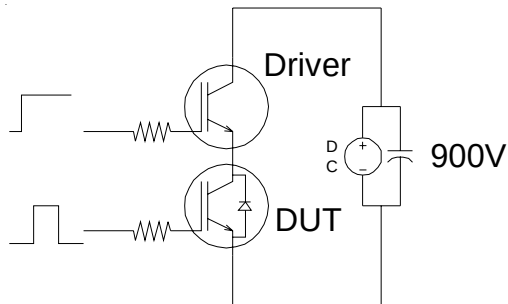
Fig.C.T.3 - RBSOA Circuit
