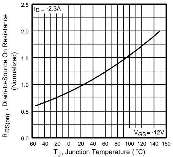
Fig 17. Normalized On-Resistance Vs. Temperature
