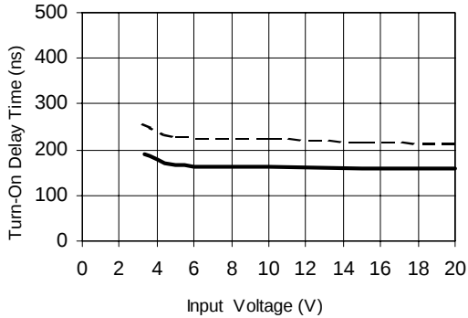
Figure 6C. Turn-On Time vs. Input Voltage
