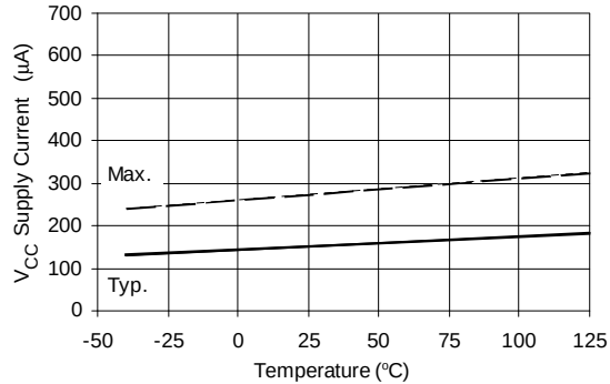
Figure 15A. Vcc Supply Current vs. Temperature
