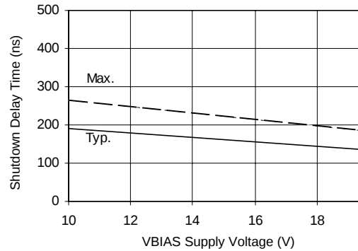
Figure 8B. Shutdown Time vs. Voltage
