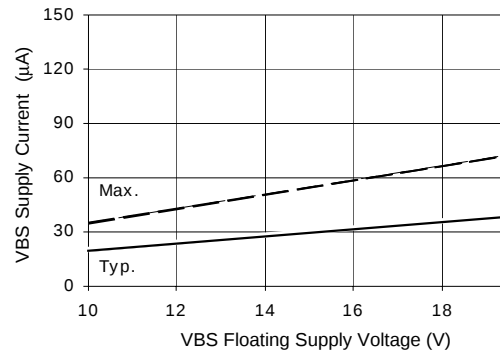
Figure 17B. V BS Supply Current vs. Voltage
