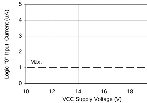
Figure 20B. Logic "0" Input Current vs. Voltage
