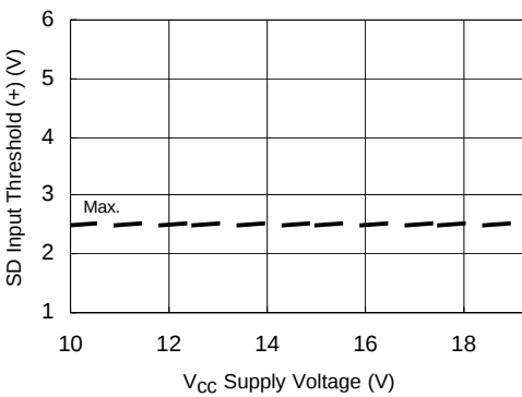
Figure 24B. SD Input Positive Going Threshold (+) vs. Supply Voltage
