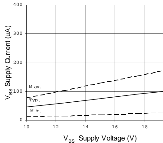
Figure 13B. V BS Supply Current vs. Supply Voltage
