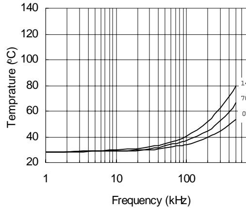
Figure 24. IRS2106 vs. Frequency (IRFBC2 R gate =33 Ω, V CC =15 V
