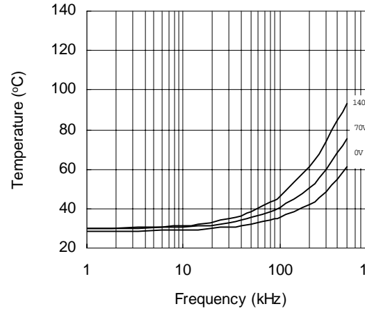
Figure 26. IRS2106 vs. Frequency (IRFBC4, R_{gate}=15 \Omega , V_{CC}=15 V
