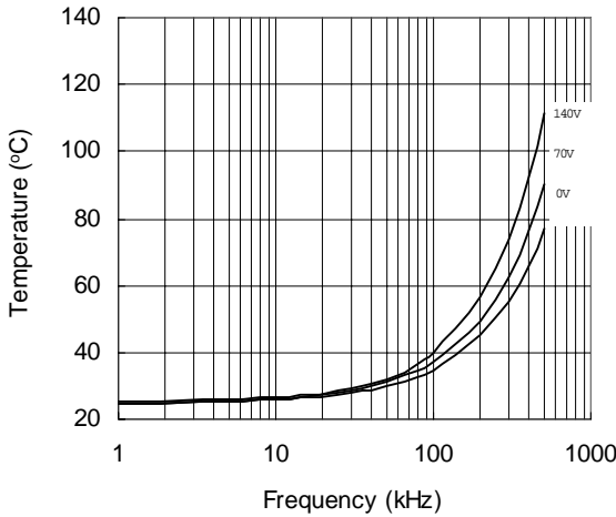
Figure 33. IRS2106S vs. Frequency (IRFBC30), R_{gate}=22 \Omega , V_{CC}=15 V
