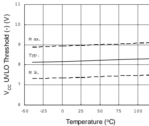
Figure 18. V CC Undervoltage Threshold (-) vs. Temperature
