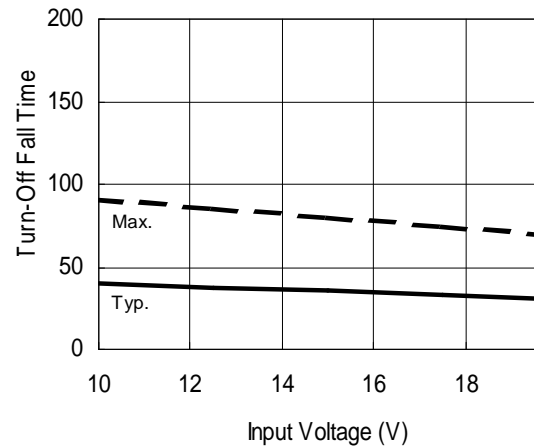
Figure 7B. Turn-Off Fall Time vs. Supply Voltage
