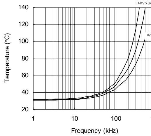
Figure 34. IRS2106S vs. Frequency (IRFBC40), R_{gate}=15 \Omega , V_{CC}=15 V
