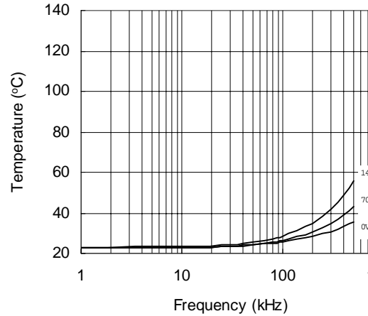
Figure 28. IRS21064 vs. Frequency (IRFBC4, R_{gate}=33 \Omega , V_{CC}=15 V
