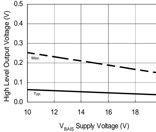
Figure 10B. High Level Output Voltage vs. Supply Voltage
