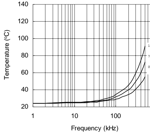
Figure 30. IRS21064 vs. Frequency (IRFBC40) R_{gate}=15 \Omega , V_{CC}=15 V
