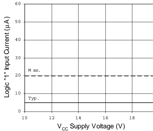
Figure 15B. Logic "1" Bias Current vs. Supply Voltage
