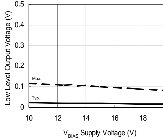
Figure 11B. Low Level Output Voltage vs. Supply Voltage
