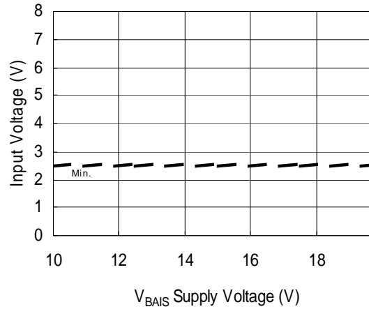
Figure 8B. Logic "1" Input Voltage vs. Supply Voltage
