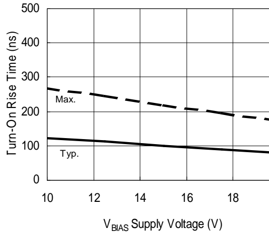
Figure 6B. Turn-On Rise Time vs. Supply Voltage
