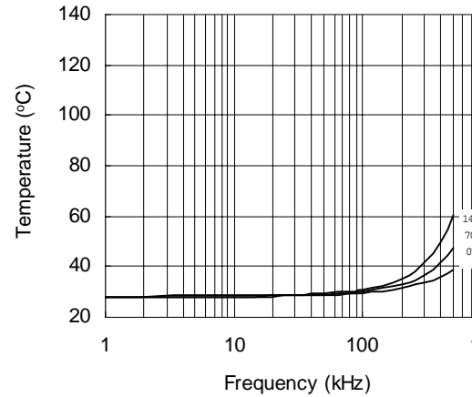
Figure 36. IRS21064S vs. Frequency (IRFBC20), R_{gate}=33 \Omega , V_{CC}=15 V
