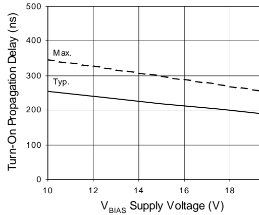
Figure 4B. Turn-On Propagation Delay vs. Supply Voltage
