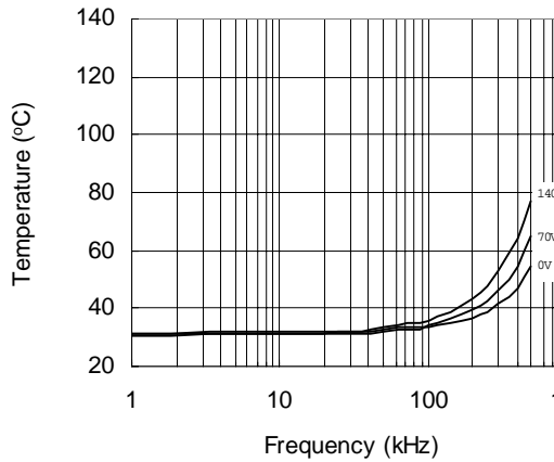
Figure 32. IRS2106S vs. Frequency (IRFBC20) R_{gate}=33 \Omega , V_{CC}=15 V
