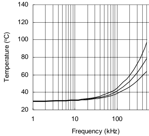
Figure 38. IRS21064S vs. Frequency (IRFBC30), R_{gate}=15 \Omega , V_{CC}=15 V
