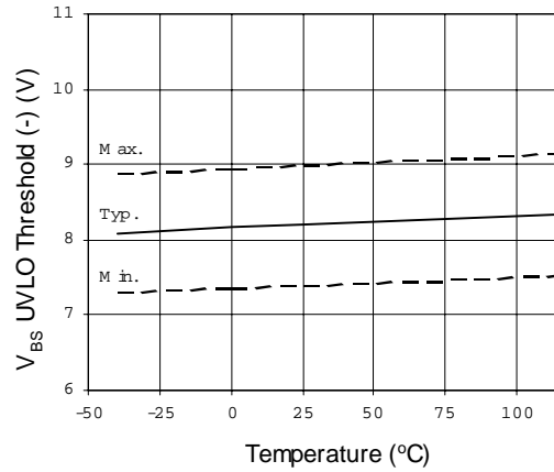
Figure 20. V_{BS} Undervoltage Threshold (-) vs. Temperature
