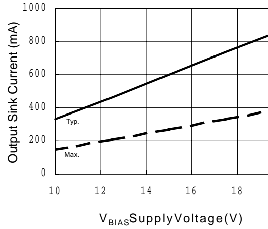
Figure 22B. Output Sink Current vs. Supply Voltage
