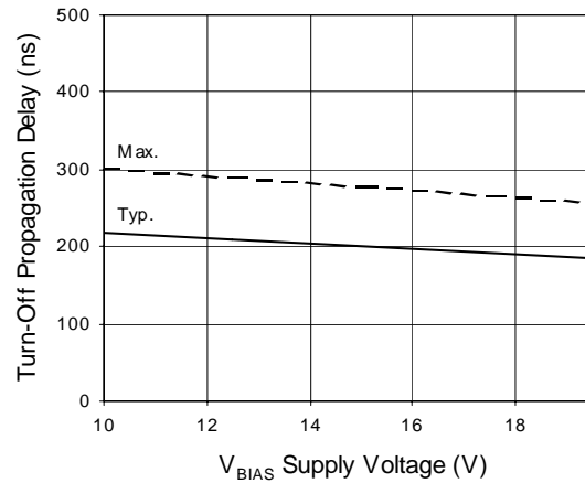
Figure 5B. Turn-Off Propagation Delay vs. Supply Voltage
