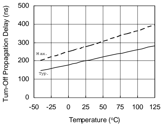
Figure 5A. Turn-Off Propagation Delay vs. Temperature
