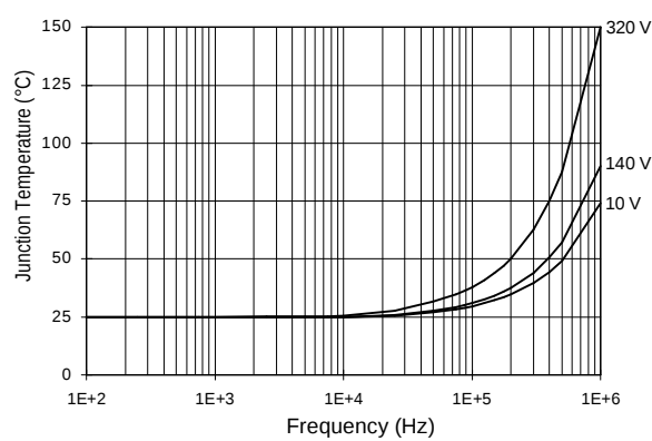
Figure 32. IRS2112S T_J vs. Frequency (IRFBC20) R_{GATE} = 33 \text{ W} , V_{CC} = 15 \text{ V}
