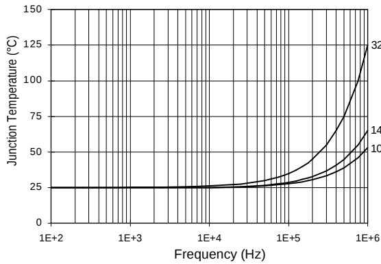
Figure 28. IRS2112 T_J vs. Frequency (IRFBC20) R_{GATE} = 33 \text{ W} , V_{CC} = 15 \text{ V}
