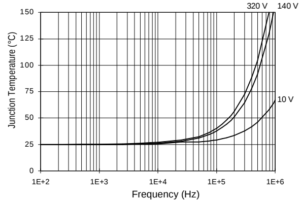
Figure 33. IRS2112S T_J vs. Frequency (IRFBC30) R_{GATE} = 22 \text{ W} , V_{CC} = 15 \text{ V}
