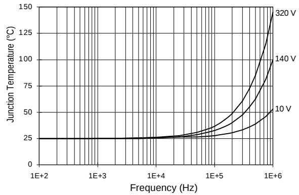
Figure 29. IRS2112 T_J vs. Frequency (IRFBC30) R_{GATE} = 22 \text{ W} , V_{CC} = 15 \text{ V}
