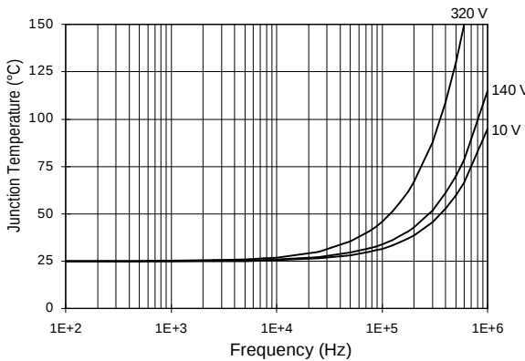
Figure 30. IRS2112 T_J vs. Frequency (IRFBC40) R_{GATE} = 15 \text{ W} , V_{CC} = 15 \text{ V}
