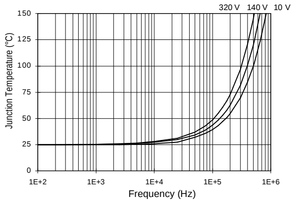
Figure 31. IRS2112 T_J vs. Frequency (IRFPE50) R_{GATE} = 10 \text{ W} , V_{CC} = 15 \text{ V}
