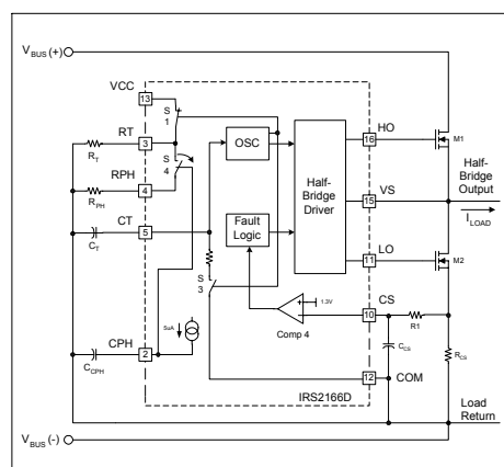
Fig.4: Ignition circuitry
