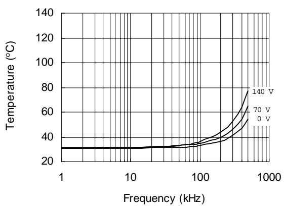
Figure 30. IRS2183S vs. Frequency (IRFBC20), R_{gate}=33 \Omega , V_{CC}=15 V
