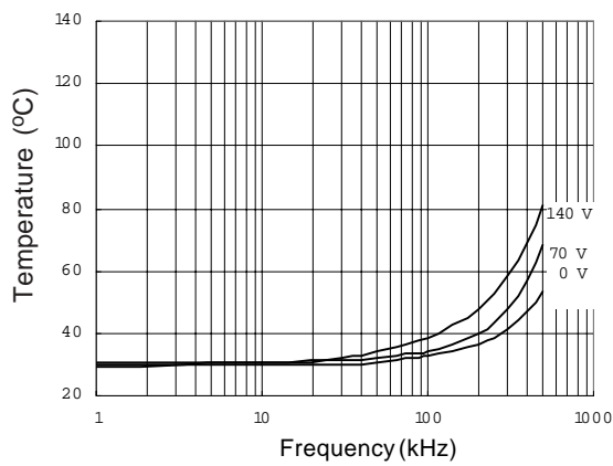
Figure 35. IRS21834S vs. Frequency (IRFBC30), R_{gate}=22 \Omega , V_{CC}=15 V
