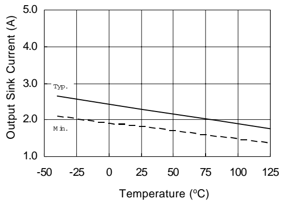
Figure 21A. Output Sink Current vs. Temperature
