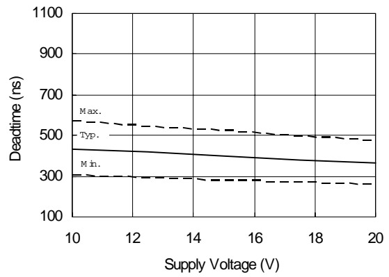
Figure 8B. Deadtime vs. Supply Voltage
