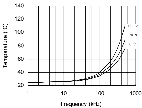
Figure 31. IRS2183S vs. Frequency (IRFBC30), R_{gate}=22 \Omega , V_{CC}=15 V
