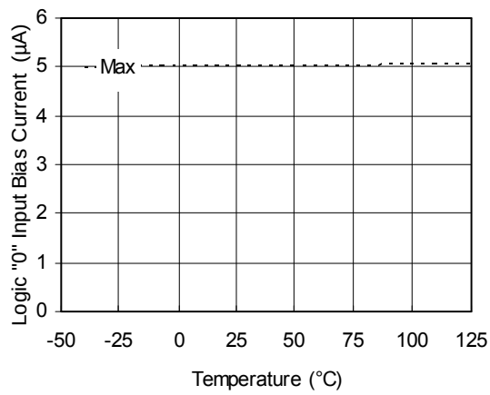
Figure 15A. Logic "0" Input Bias Current vs. Temperature
