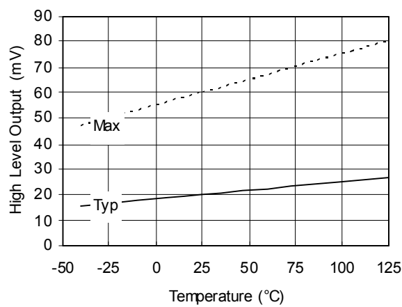
Figure 9A. High Level Output vs. Temperature ( I_O = 2 \text{ mA} )
