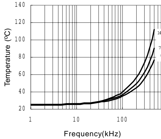
Figure 30. IRS2186S vs. Frequency (IRFBC20), R_{gate} = 22 \Omega , V_{CC} = 15 V
