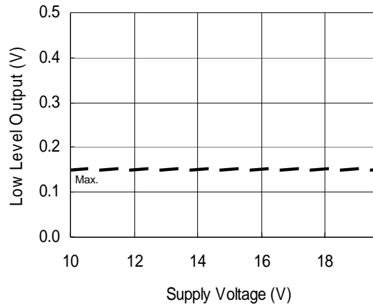
Figure 11B. Low Level Output vs. Supply Voltage
