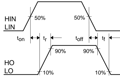
Figure 2. Switching Time Waveform Definition
