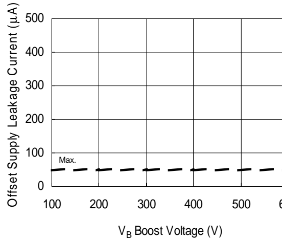
Figure 12B. Offset Supply Leakage Current vs. V B Boost Voltage
