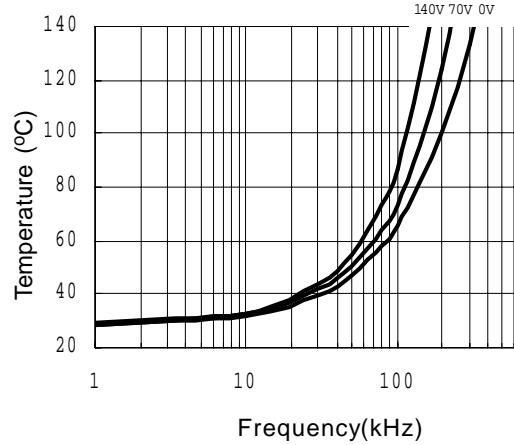
Figure 32. IRS2186S vs. Frequency (IRFBC40), R_{gate} = 10 \Omega , V_{CC} = 15 V
