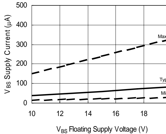
Figure 13B. V BS Supply Current vs. V BS Floating Supply Voltage
