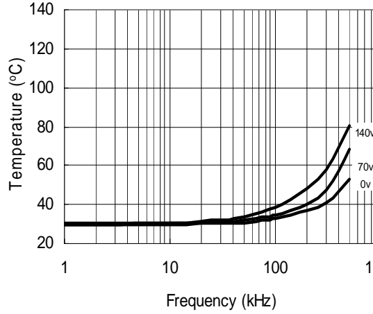
Figure 34. IRS21864S vs. Frequency (IRFBC30), R_{gate}=22 \Omega , V_{CC}=15 V
