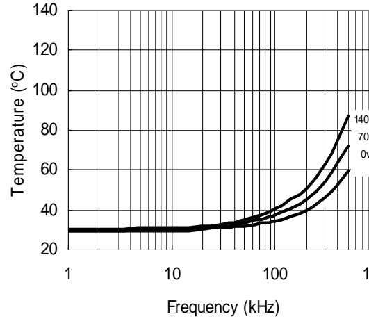
Figure 22. IRS2186 vs. Frequency (IRFBC30) R_{gate}=22 \Omega, V_{CC}=15 V
