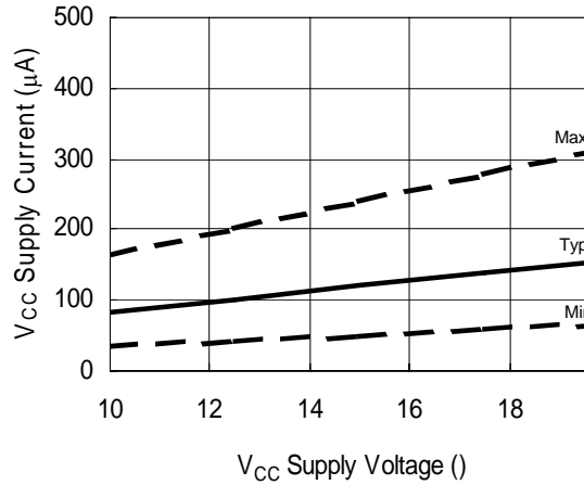
Figure 14B. V_{CC} Supply Current vs. Supply Voltage
