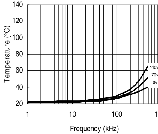
Figure 26. IRS21864 vs. Frequency (IRFBC30), R gate =22 Ω, V CC =15 V
