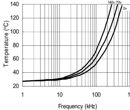
Figure 36. IRS21864S vs. Frequency (IRFPE50), R_{gate}=10 \Omega , V_{CC}=15 V
