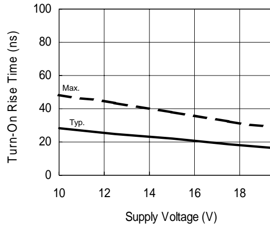
Figure 6B. Turn-On Rise Time vs. Supply Voltage
