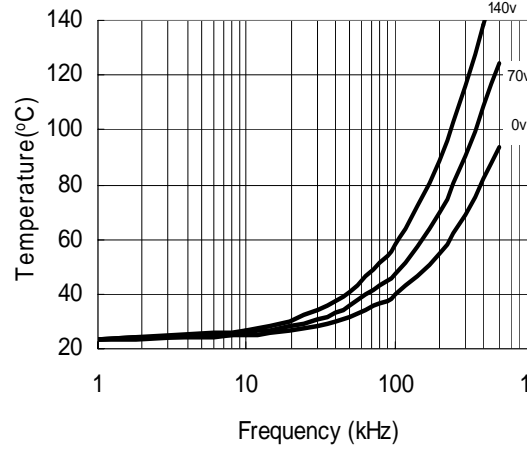
Figure 28. IRS21864 vs. Frequency (IRFPE50), R gate =10 Ω, V CC =15 V
