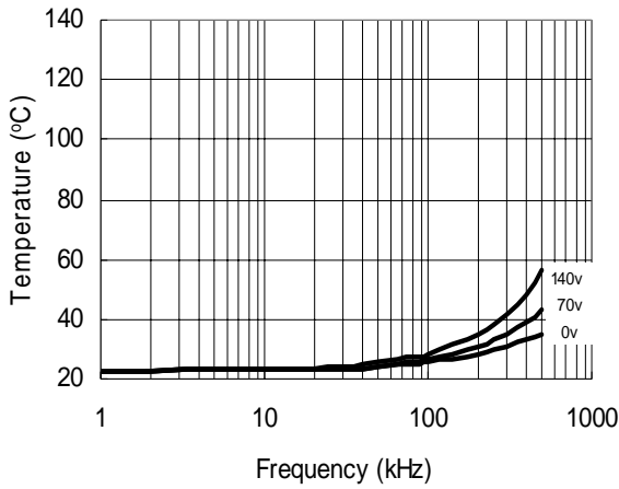
Figure 25. IRS21864 vs. Frequency (IRFBC20), R gate =33 Ω, V CC =15 V
