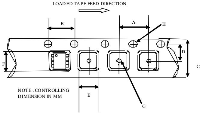
CARRIER TAPE DIMENSION FOR 8SOIC
