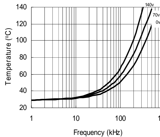
Figure 24. IRS2186 vs. Frequency (IRFPE50) R_{gate}=10 \Omega, V_{CC}=15 V
