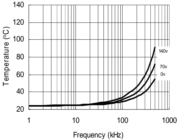
Figure 27. IRS21864 vs. Frequency (IRFBC40), R gate =15 Ω, V CC =15 V
