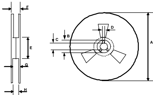
REEL DIMENSIONS FOR 8SOIC
