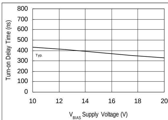
Figure 2B. Turn-On Time vs. Supply Voltage
