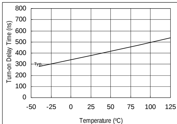
Figure 2A. Turn-On Time vs. Temperature
