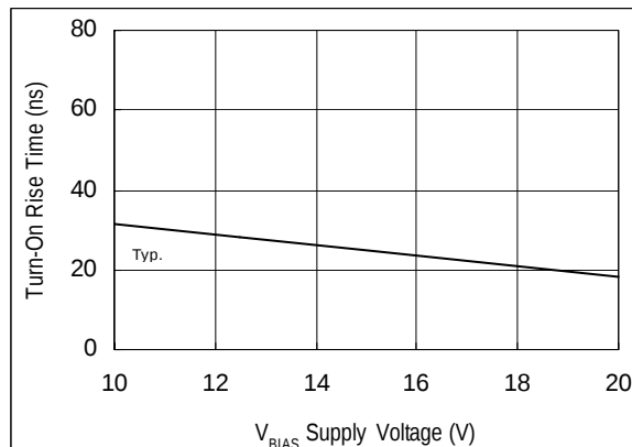
Figure 4B. Turn-On Rise Time vs. Supply Voltage
