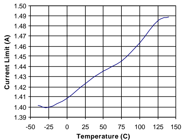
Figure 15 - Typical Current Limit vs. Temperature ( V_{IN}=5.5\text{V} )
