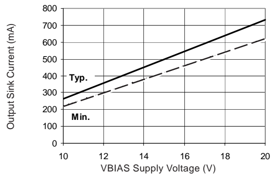
Figure 32B Output Sink Current vs Voltage
