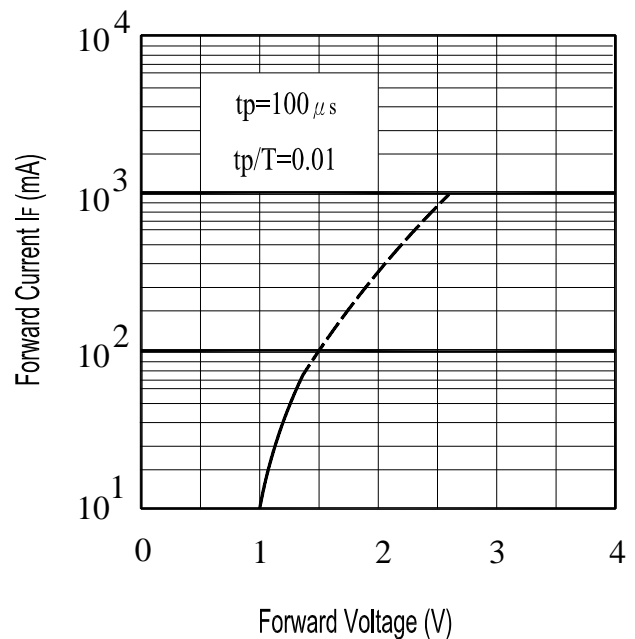
Fig.4 Forward Current
