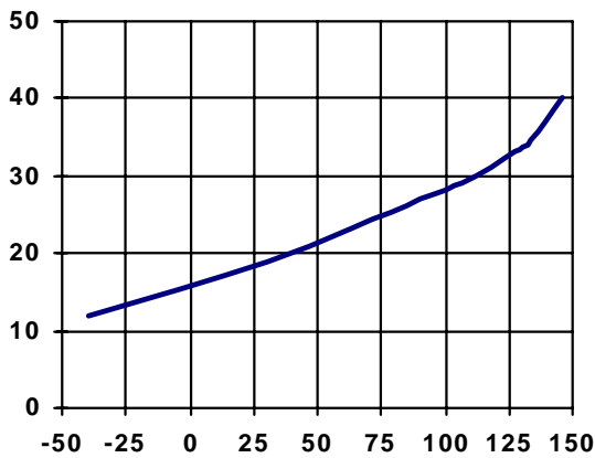
Figure 7 - I_{ccoff} ( \mu\text{A} ) vs T_j ( ^{\circ}\text{C} )
