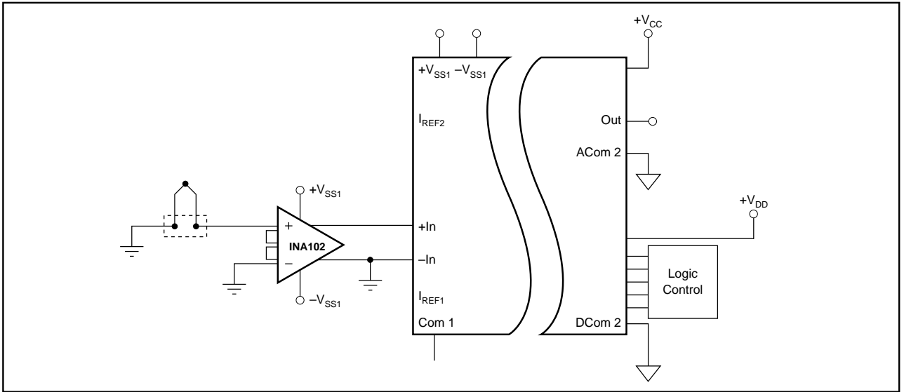
FIGURE 18. Temperature Measurement Using Thermocouple with Small Span.
