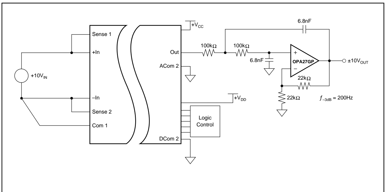
FIGURE 15. Isolated Voltage Measurement Channel with Output Filter.
