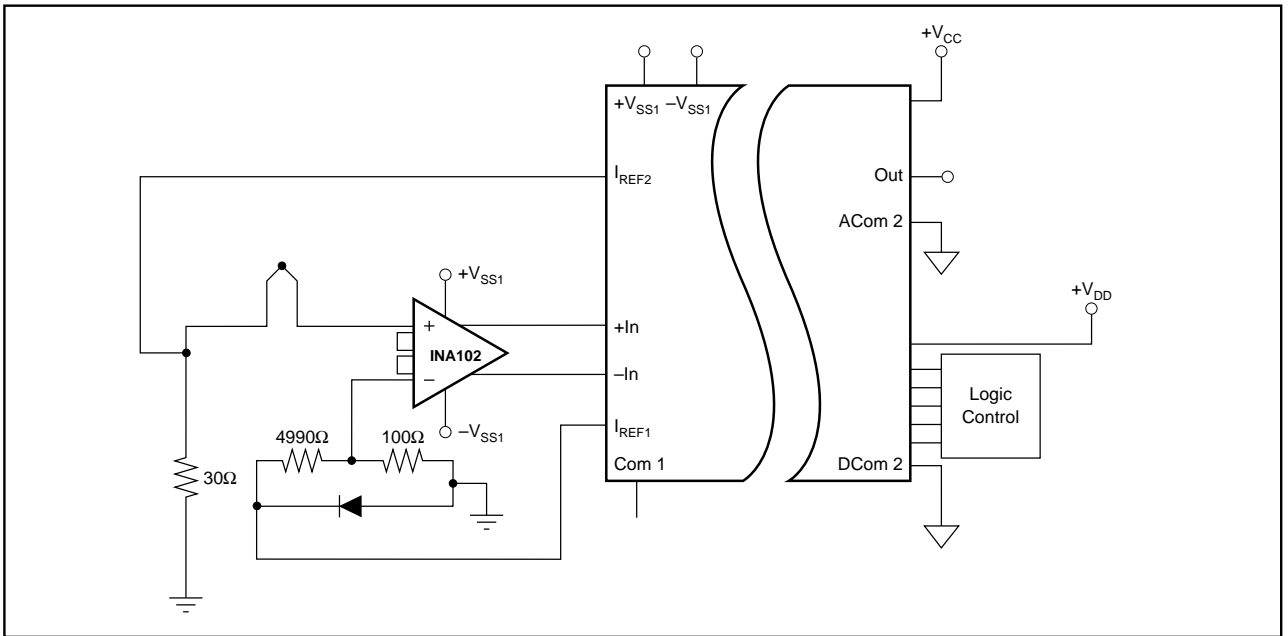
FIGURE 19. Thermocouple with Cold Junction Compensation.
