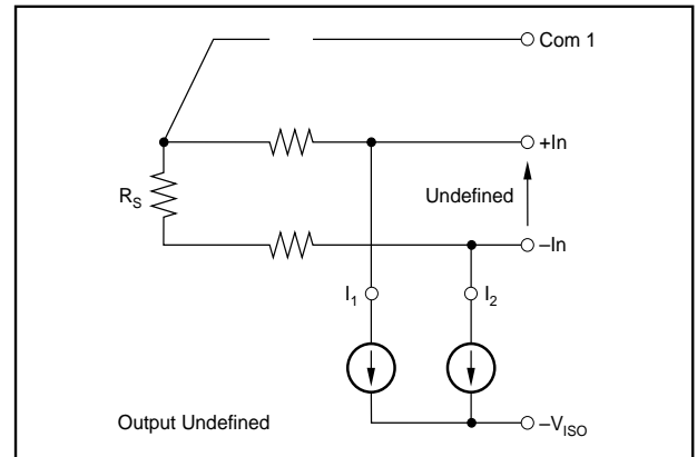
FIGURE 14. Com 1 Open Circuit.
