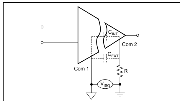
FIGURE 2. Barrier Capacitance.
