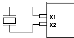
FIGURE 7. RECOMMENDED CRYSTAL CONNECTION
